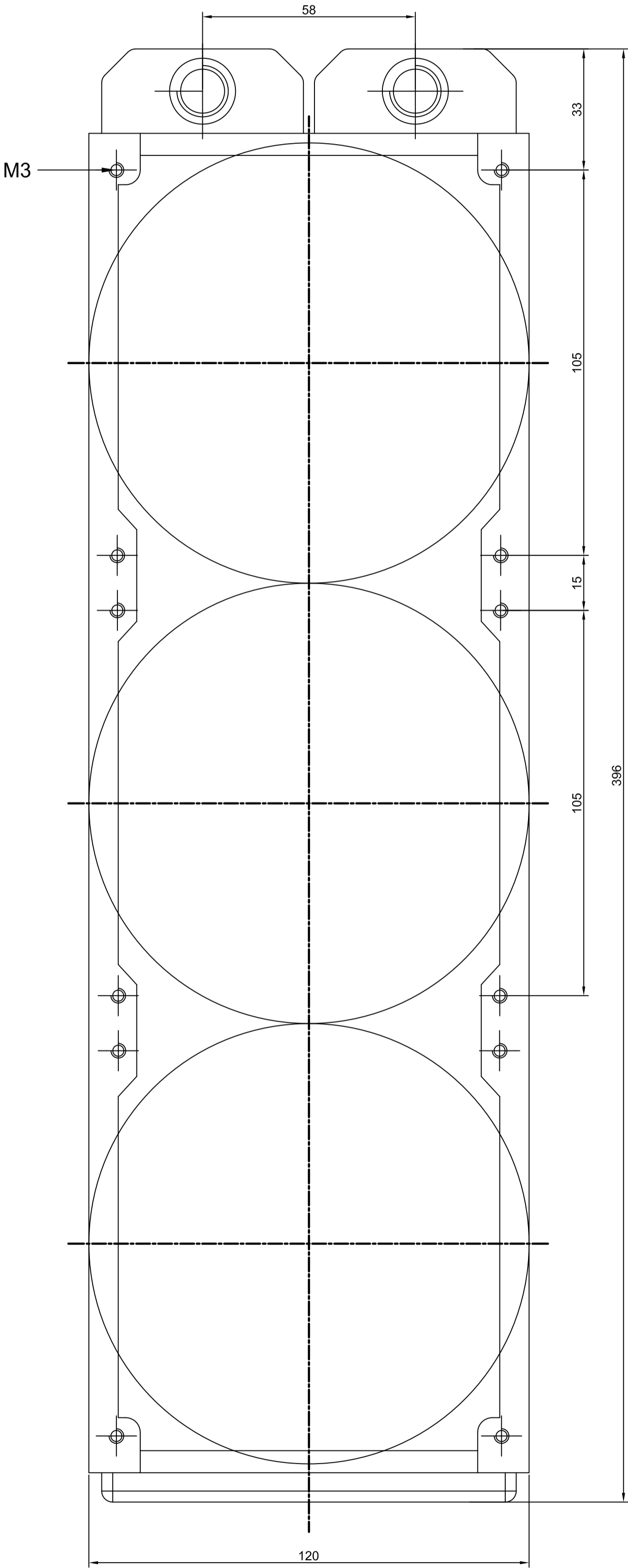
EK-COOLSTREAM RAD XT 360 template by EKWB (scale 1:1)
