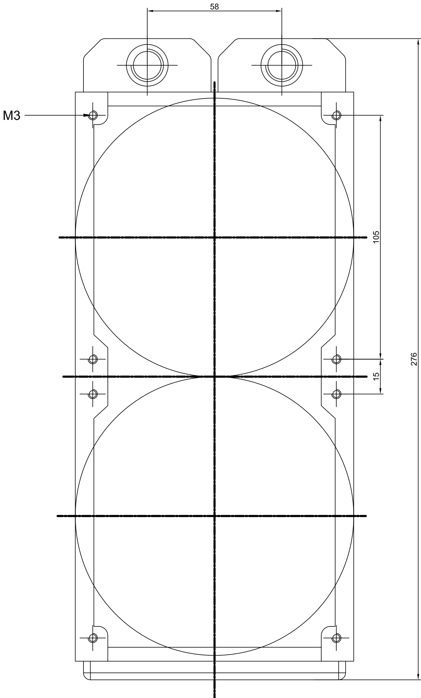
EK-COOLSTREAM RAD XT 240 template by EKWB (scale 1:1)
