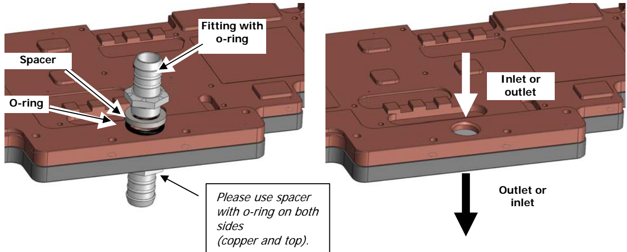
Picture 1: Sample picture of fitting installation.
