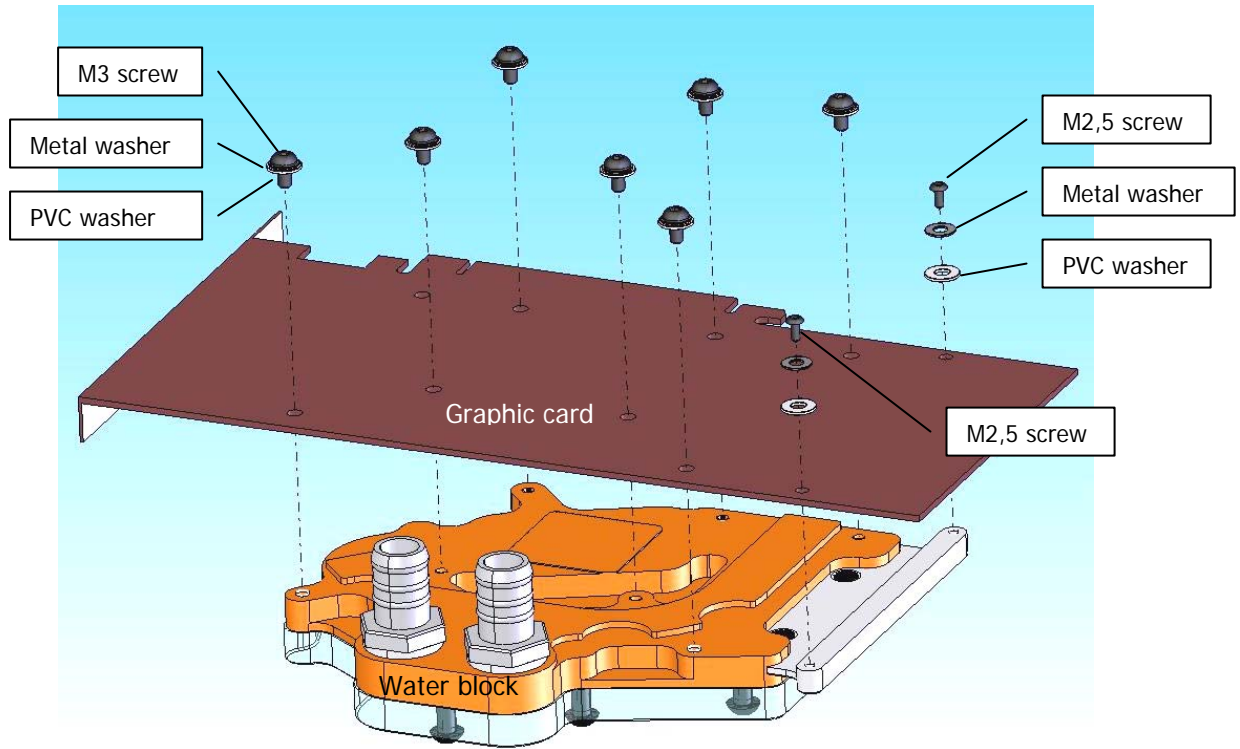
Picture 2: Mounting installation:
