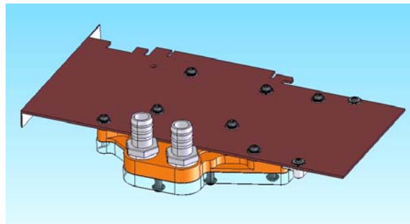
Picture 3: Installed water block on Radeon X1800 series graphic card.
