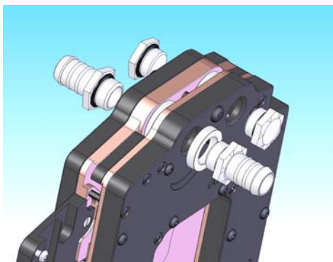
Picture 3: Installing fittings, plugs and spacers,
