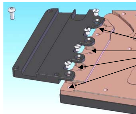
Picture 4: Alu part for mosfets
