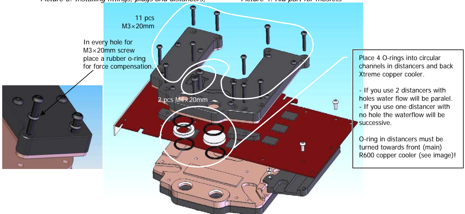
Picture 5: Radeon HD2900 TX series graphic card with assembling view - front side.
