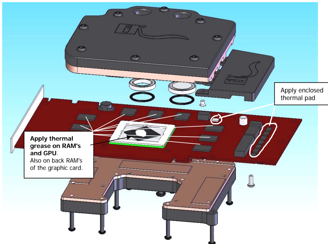
Picture 6: Radeon HD2900 TX series graphic card with assembling view - front side.
